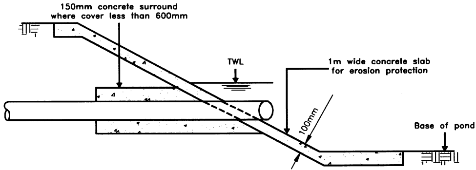
Figure 5.7 Inlet structure for secondary facultative and maturation ponds. This would receive the discharge from the outlet structure shown in Figure 5.8.
